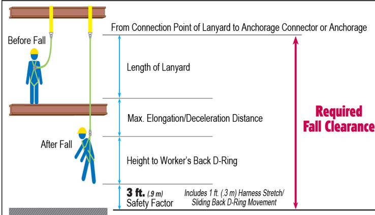
Illustration: Shock-Absorbing Lanyard with Cross-Arm Strap Anchorage Connector
