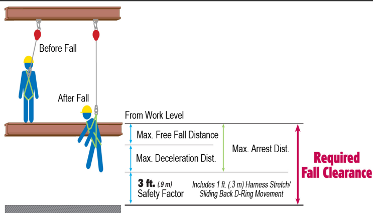
Illustration: Self-Retracting Lifeline with D-Bolt Anchorage Connector
